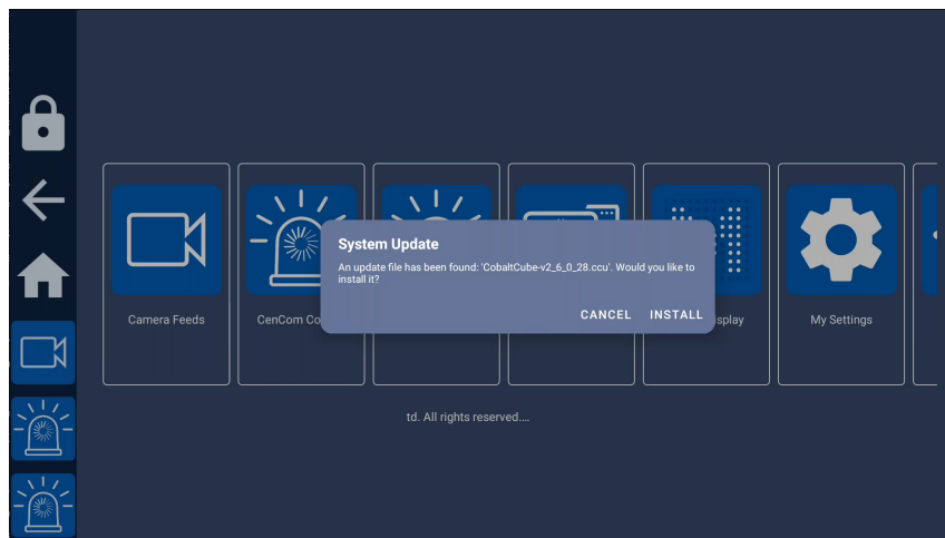
Figure 7: Update dialog
