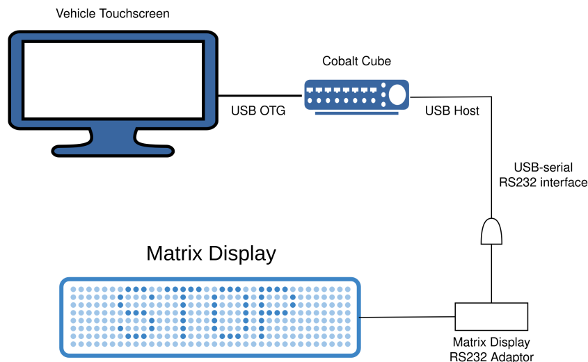
Figure 2: Connectivity diagram for the Matrix Display
