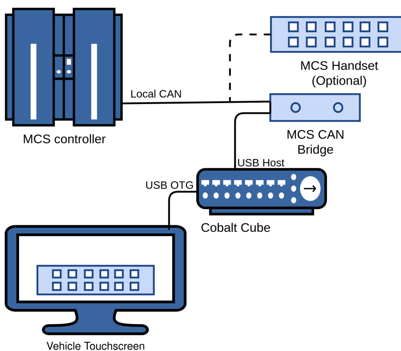
Figure 1: MCS Control connectivity diagram
